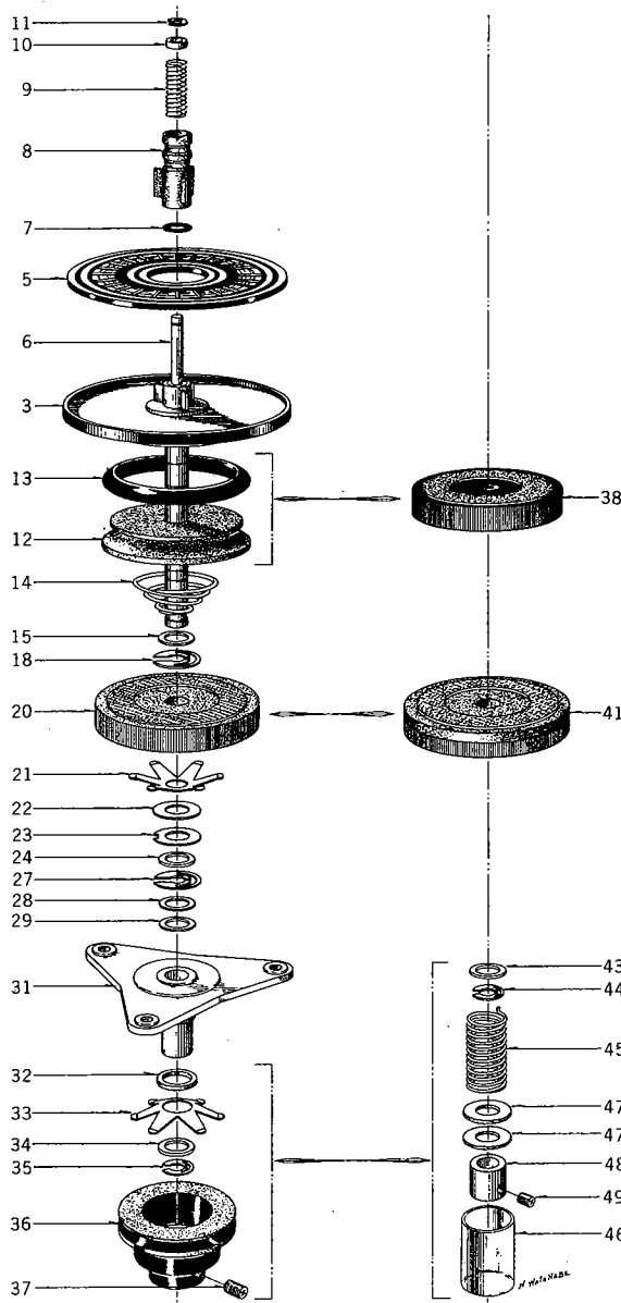
FIG. 2 ILLUSTRATION OF REEL TABLE BLOCK
